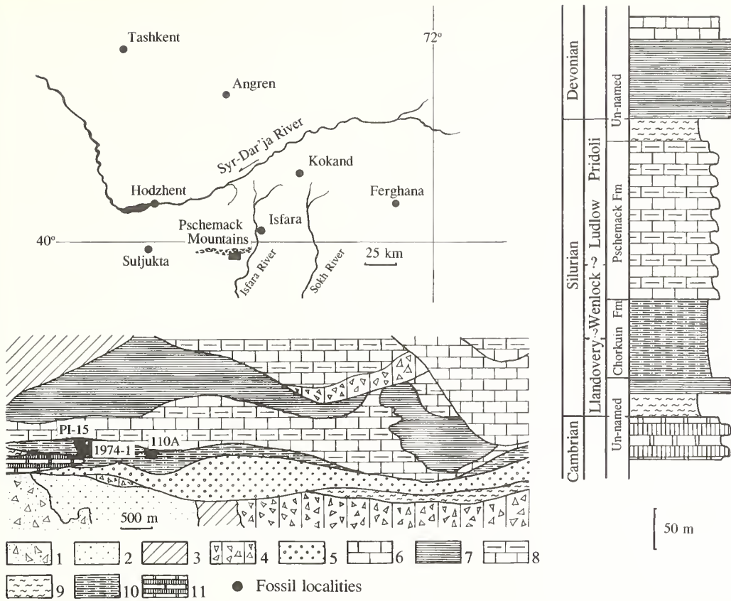
TEXT-FIG. 1. Derivation of Isfari spir a septata gen. et sp. nov. from the Chorkuin Formation of the Pskemack Mountains, Central Asia; localities are discussed in the text. Lithologies: 1, alluvial deposits; 2, sandstones and gritstones; 3, clays; 4, olistostromes; 5, conglomerates; 6, dolomitic limestones; 7, black cherts; 8, alternations of limestones, clayey limestones and shales; 9, clay shales; 10, siltstones; 11, alternations of cherty rocks and dolomites.
